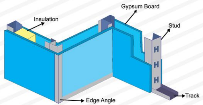
Assembled Partition
